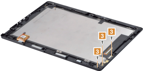
Figure 9. Removal steps of power board and audio board (continued)
